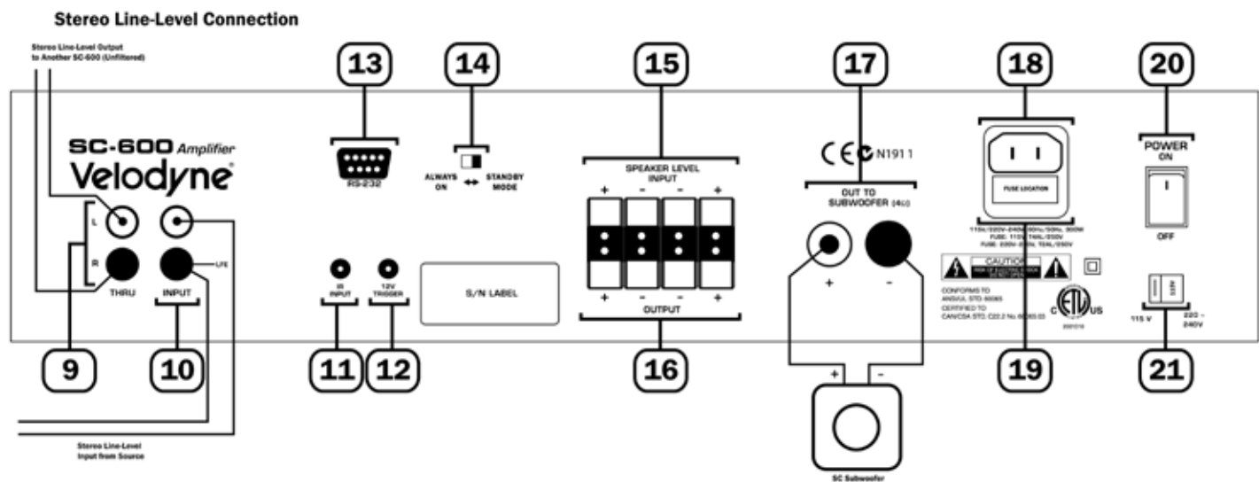
Figure 2B: Stereo Line-Level Connection.
