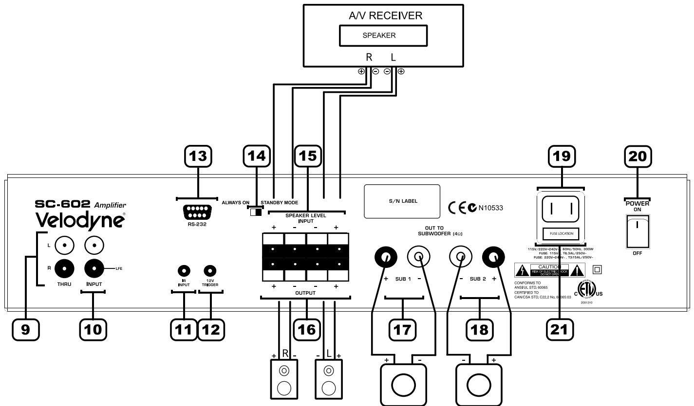
Figure 3: Speaker-Level Connection.
